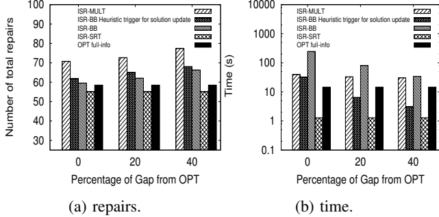
Fig. 5: Trade-off between execution time and repairs.
